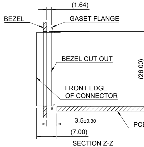
SECTION Z-Z
