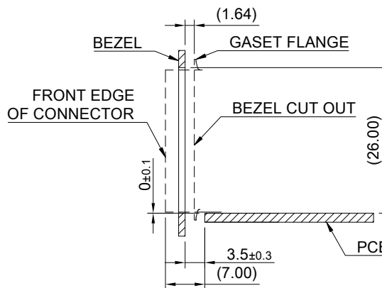
SECTION Z-Z
