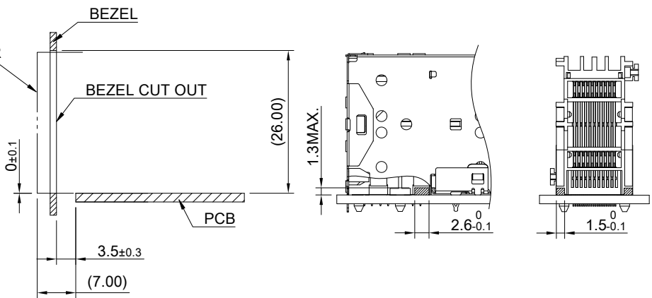
SECTION Z-Z LED CLEARANCE REQUIREMENTS
