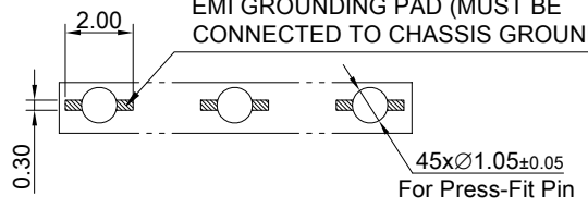
DETAIL C SCALE 4:1
