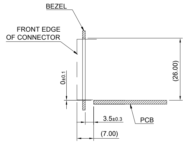
SECTION Z-Z
