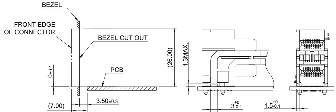
SECTION Z-Z
