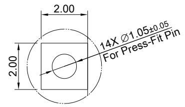
DETAIL D SCALE 3:1
