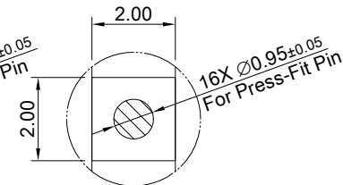
DETAIL J SCALE 3:1
