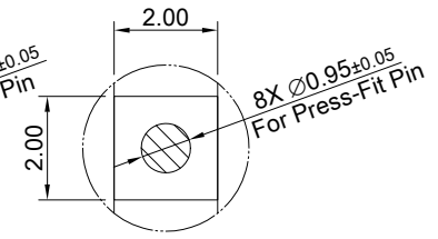
DETAIL F SCALE 3:1
