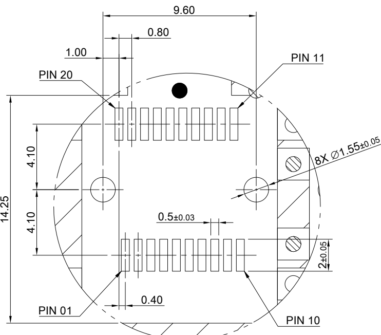
DETAIL G SCALE 2:1
