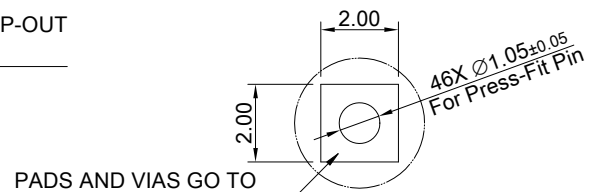
DETAIL E SCALE 4:1
