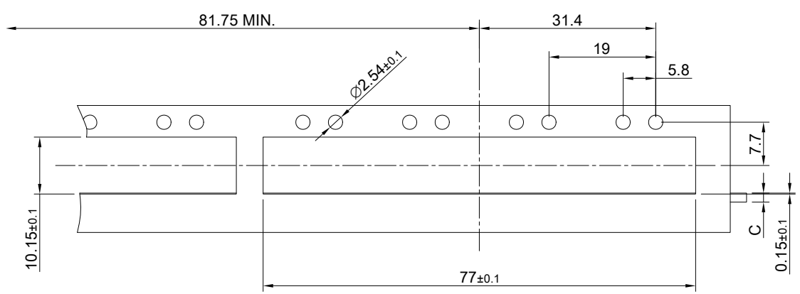
SINGLE-SIDE CONFIGURATION
