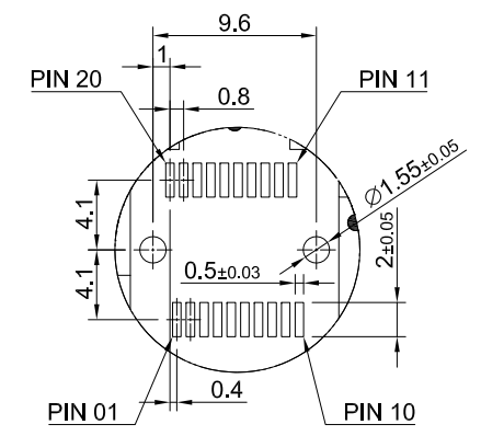
DETAIL D SCALE 2:1
