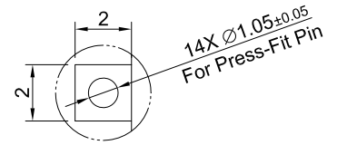
DETAIL B SCALE 4:1
